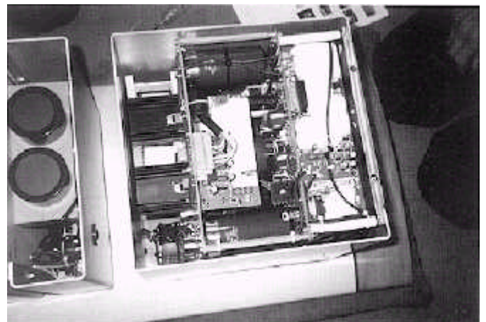
Fig 2: The bottom compartment of the twin-towered construction is the first door to the switch mode power supply. Materials that painted in white on the circuit board are used for cooling. There's a black round object located under the bottom of top compartment, and that is the never-before-seen air pressure switch.
