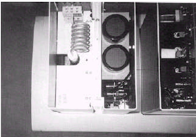
Fig 1: Coaxial solid output copper tube through the shield box of input stage. The exquisite spiral construction should be the output filter section, which takes the advantage of inductive effect.
